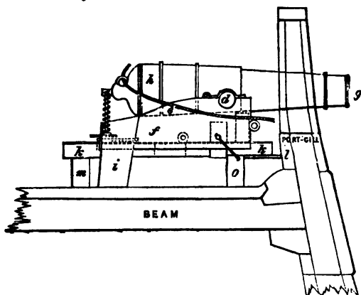
Fig. 4. —Section of the Port and Carronade.
