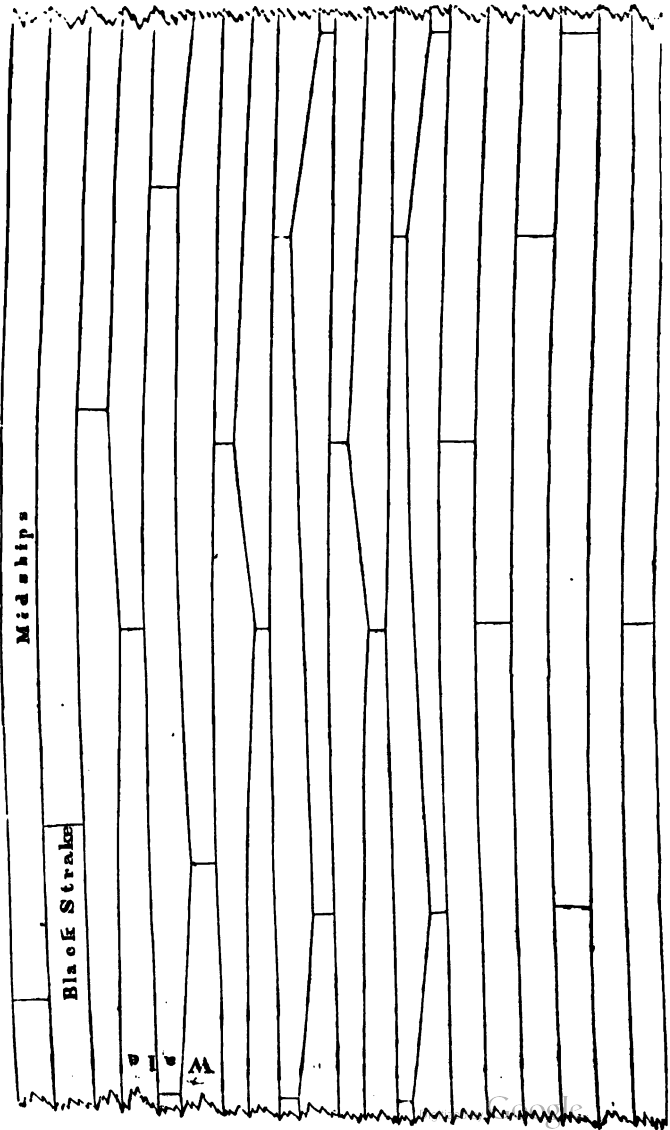
Sketch 2. Expansion of Plank. Midship Body.
