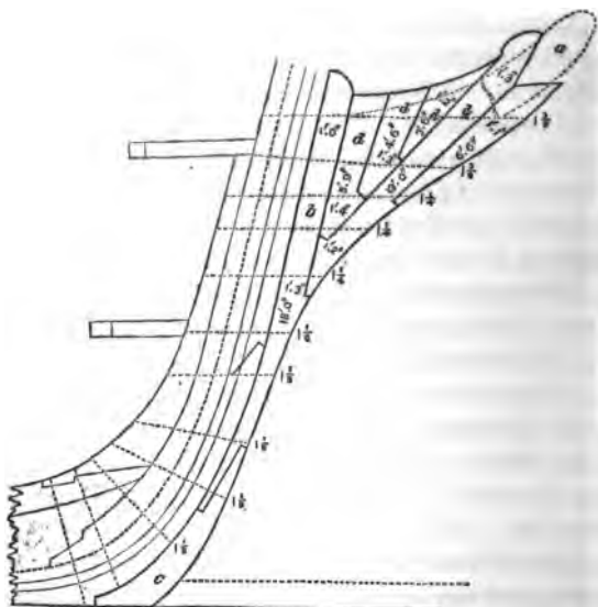
a , Figure head. b , Independent piece. c , Gripe. d , Chocks to fill up the knee.
