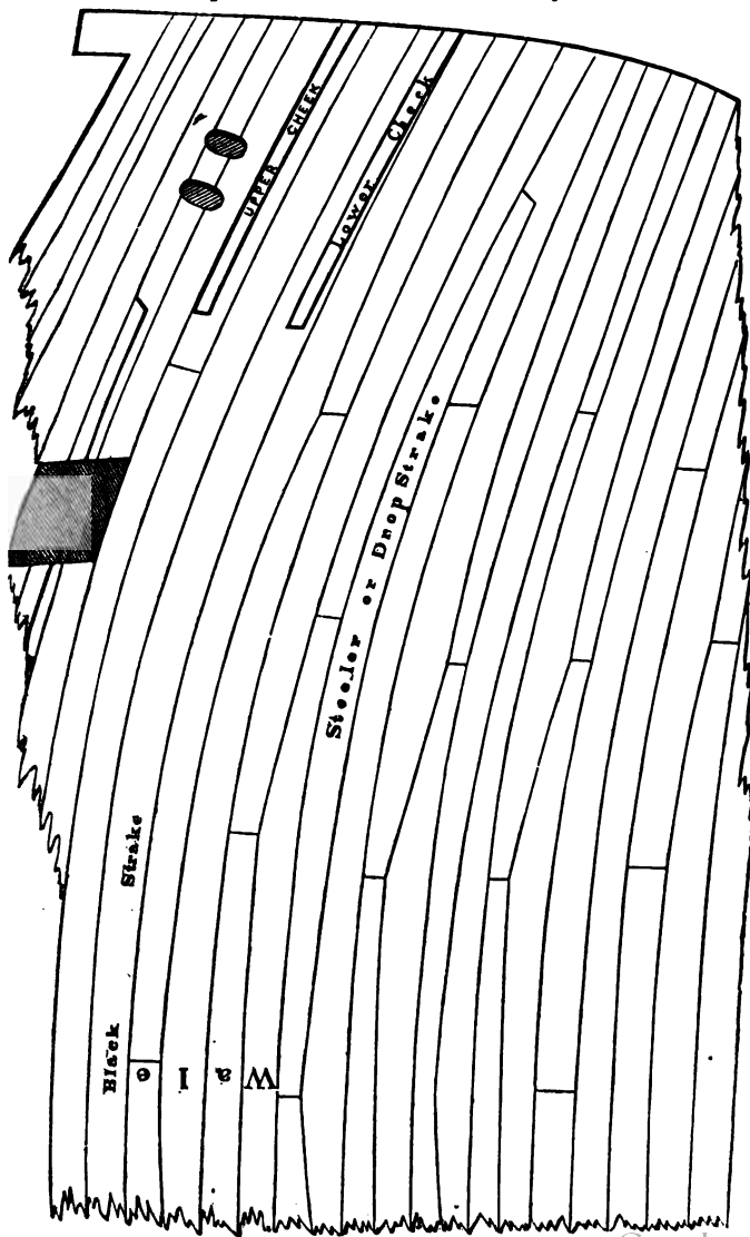
Sketch 1. Expansion of Plank outside. Fore Body.
