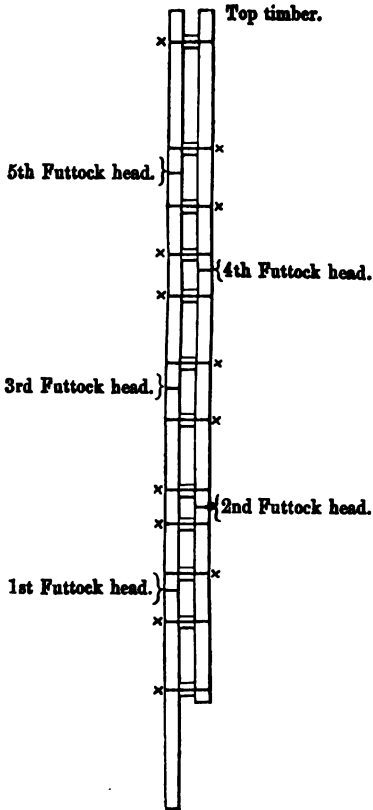
Frame Bolts and Chocks marked x.
